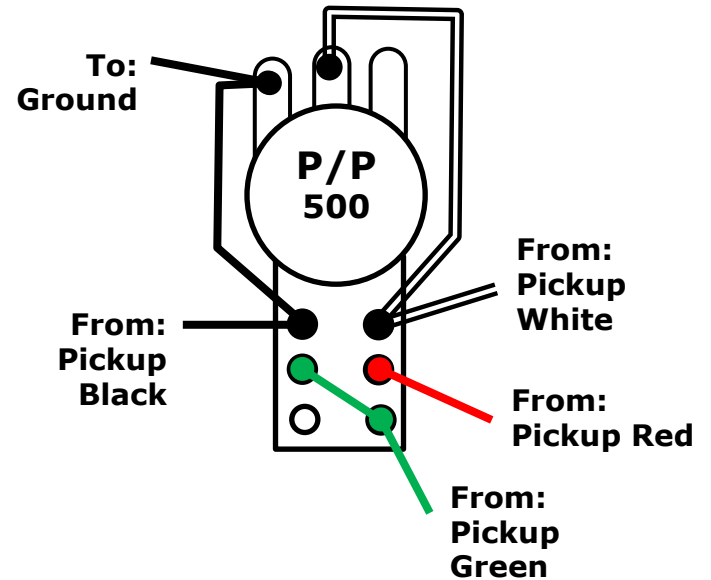
J Bass Push/Pull Pot (DPDT switch) Detail
