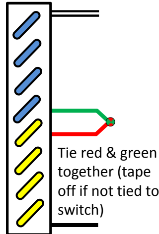
Normal (Series) Operation
